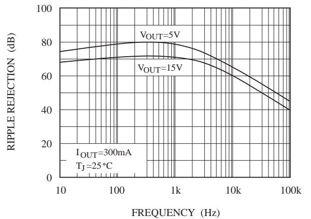
RIPPLE REJECTION
