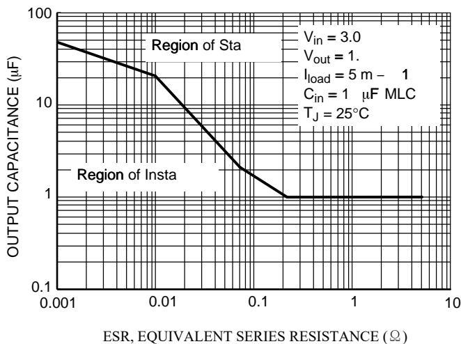
Output Capacitance vs. ESR
