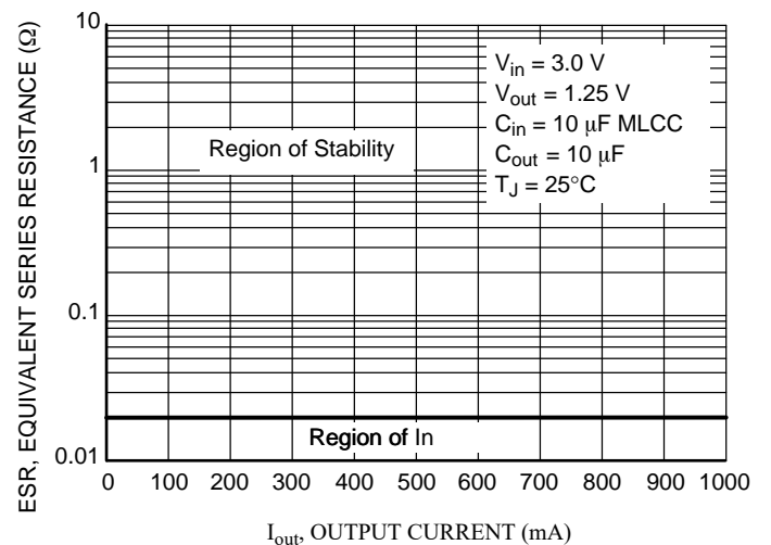
Typical ESR vs. Output Current
