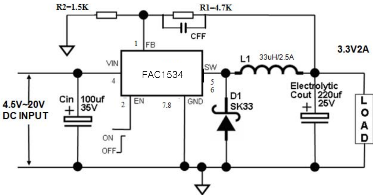
Fig11. FAC1534 Typical Application Circuit @ 3.3V/2A
