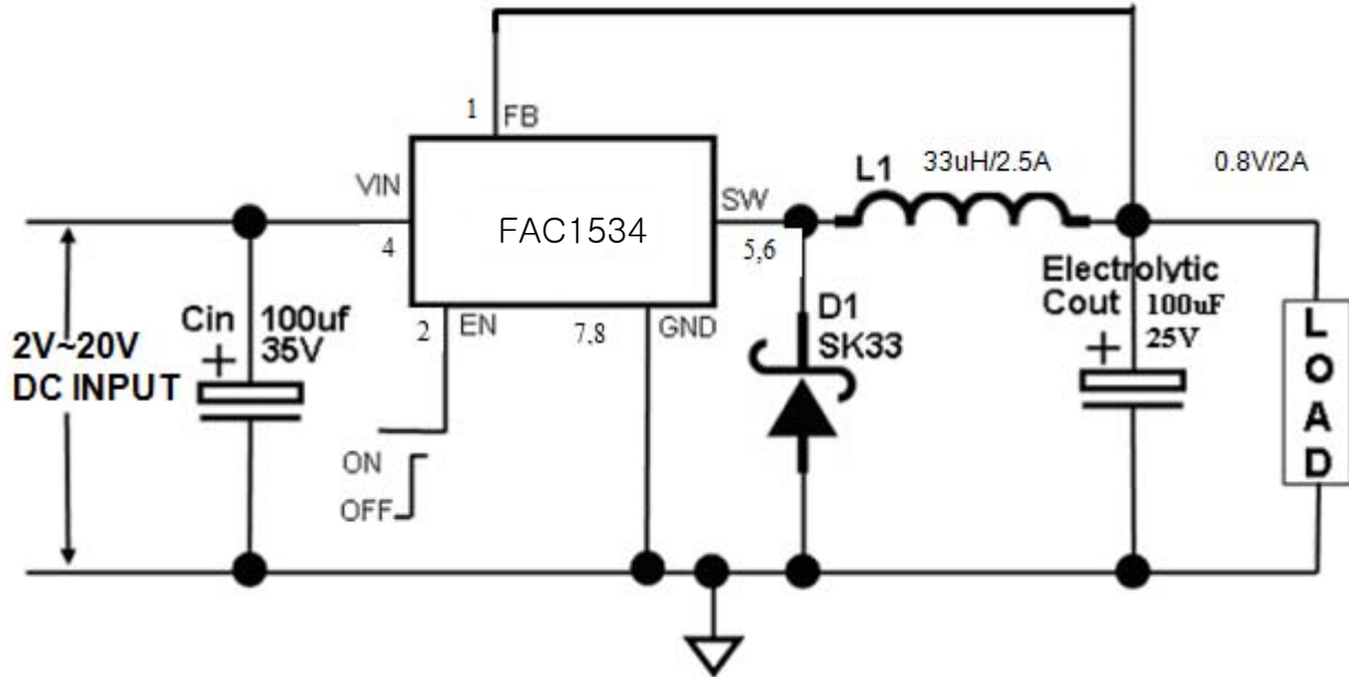
Fig8. FAC1534 Typical Application Circuit @ 0.8V/2A
