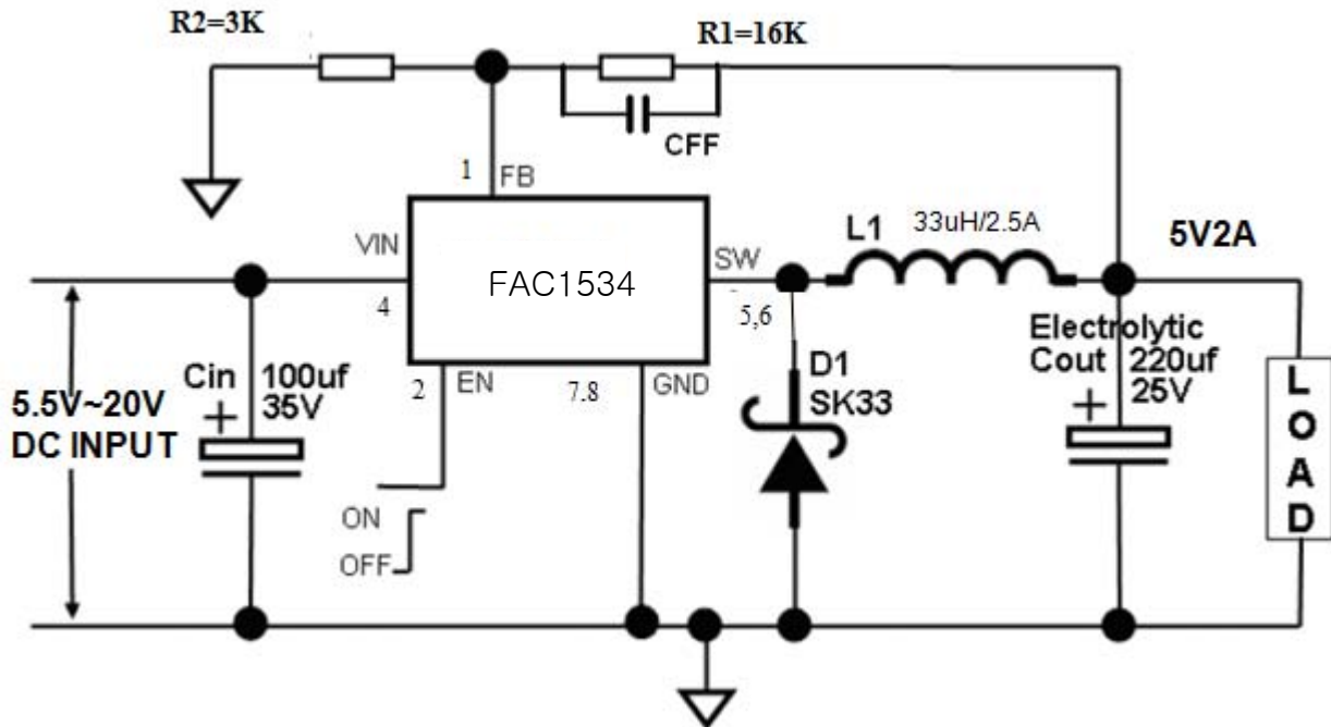
Fig10. FAC1534 Typical Application Circuit @ 5V/2A
