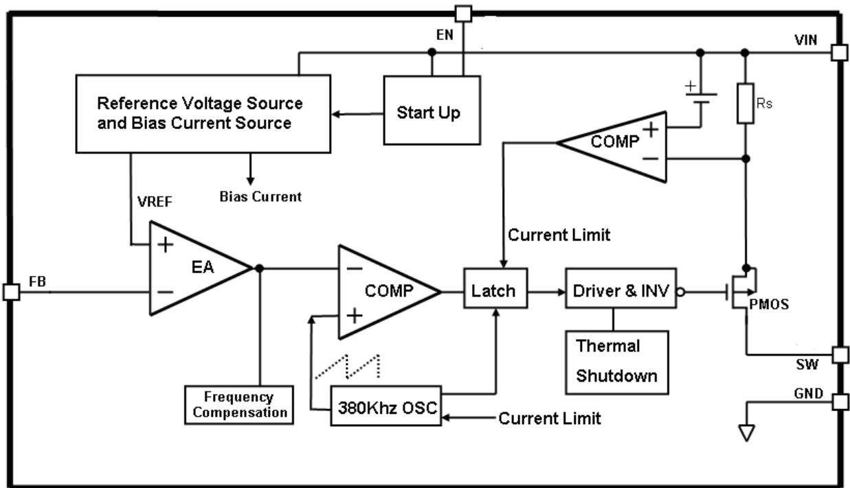
Figure 3 Function Block Diagram of FAC1534
