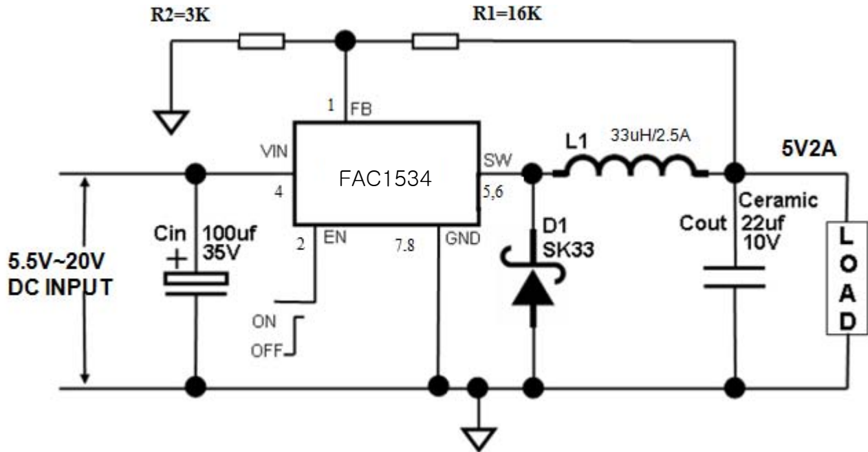
Fig12. FAC1534 Typical Application Circuit (with ceramic output capacitor) @ 5V/2A
