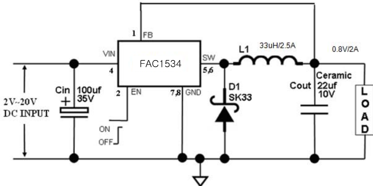
Fig9. FAC1534 Typical Application Circuit (with ceramic output capacitor) @ 0.8V/2A
