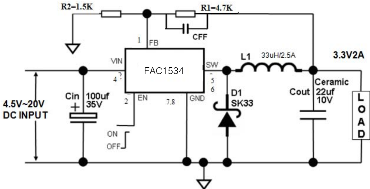
Fig13. FAC1534 Typical Application Circuit (with ceramic output capacitor) @ 3.3V/2A
