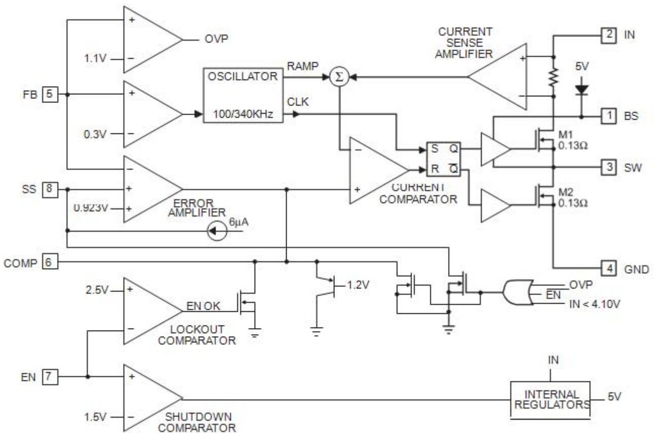
Figure 3 Function Block Diagram of FAC1482F
