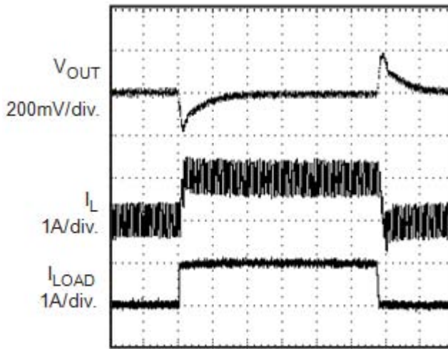
Figure 12. Load Transient
