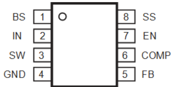
Figure 2 Pin Configuration of FAC1482F(Top View)
