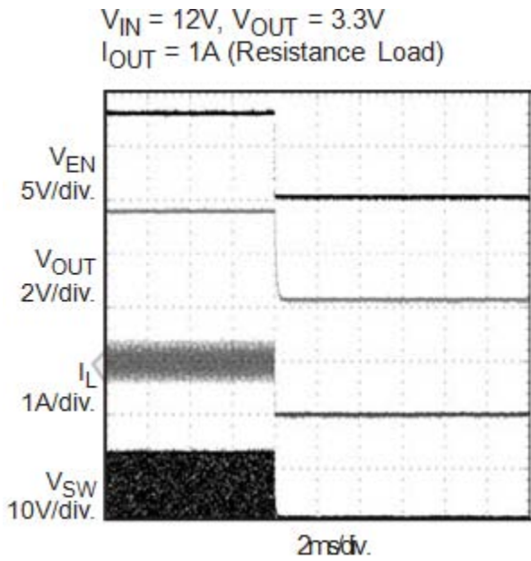
Figure 6. Shutdown through Enable
