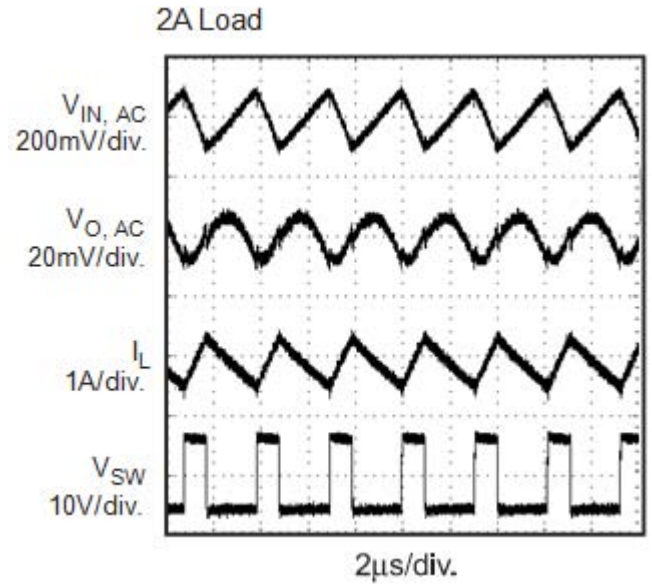
Figure 7. Heavy Load Operation
