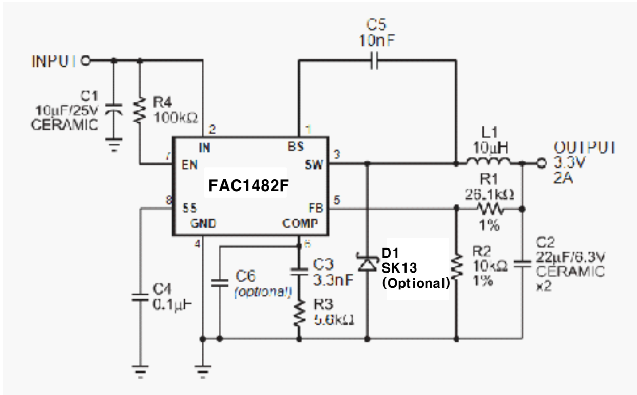
Fig13. FAC1482F with 3.3V Output, 22µF/6.3V Ceramic Output Capacitor
