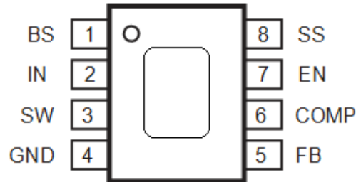
Figure 2 Pin Configuration of FAC1484(Top View)
