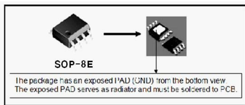
Figure 1. Package Types of FAC1484
