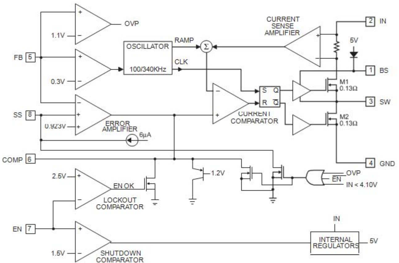
Figure 3 Function Block Diagram of FAC1484
