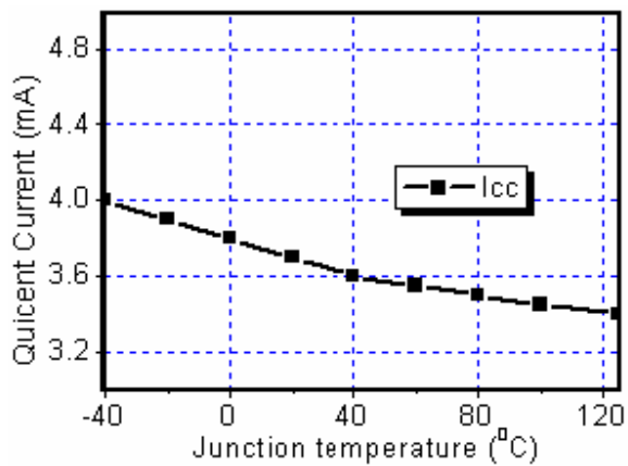
Figure 6. Icc vs. Temperature
