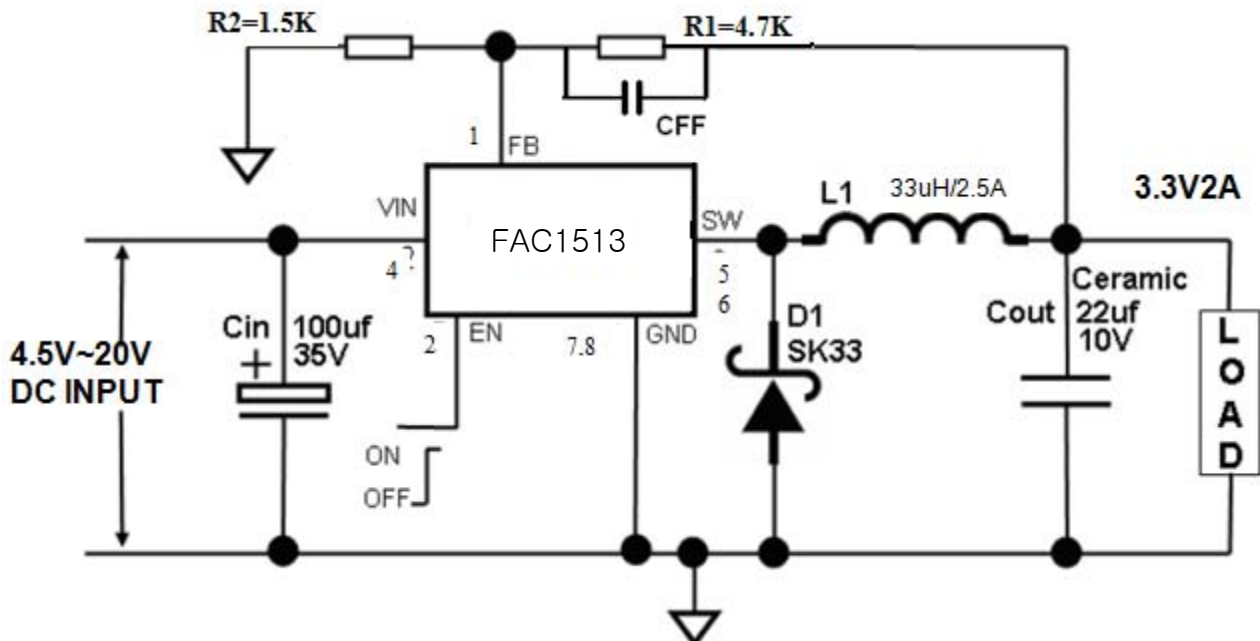
Fig13. FAC1513 Typical Application Circuit (with ceramic output capacitor) @ 3.3V/2A
