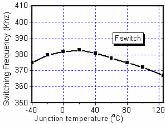
Figure 4. Switching Frequency vs. Temperature
