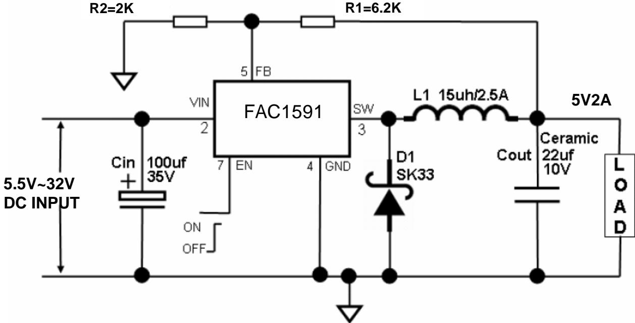
Fig10. FAC1591 Typical Application Circuit (with ceramic output capacitor) @ 5V/2A
