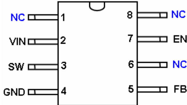
Figure 2 Pin Configuration of FAC1591 (Top View)
