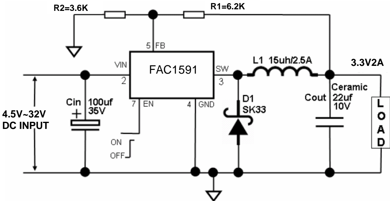
Fig11. FAC1591 Typical Application Circuit (with ceramic output capacitor) @ 3.3V/2A
