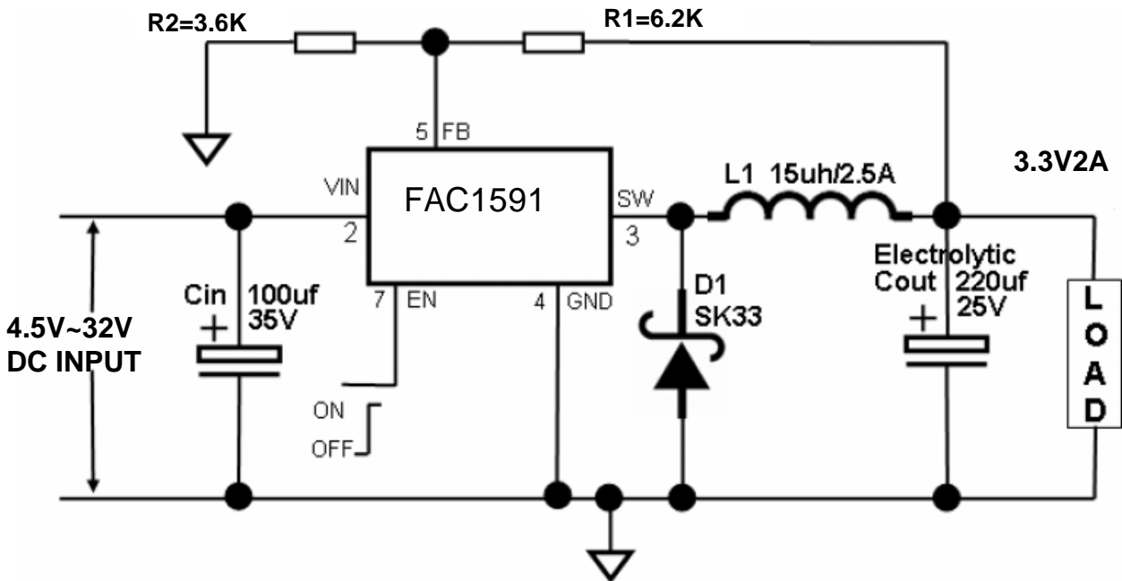
Fig9. FAC1591 Typical Application Circuit @ 3.3V/2A
