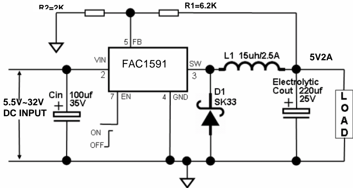
Fig8. FAC1591 Typical Application Circuit @ 5V/2A
