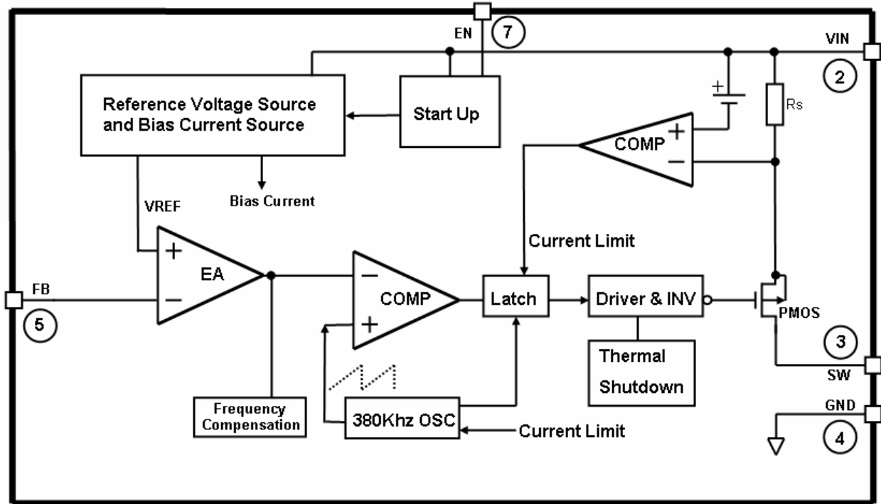
Figure 3 Function Block Diagram of FAC1591
