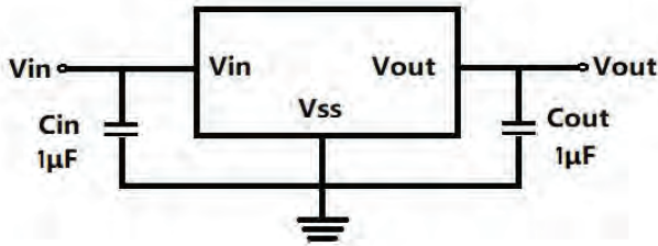
Figure1 FC6107A Typical Application Circuit
