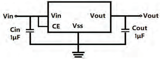
Figure2 FC6107B Typical Application Circuit
