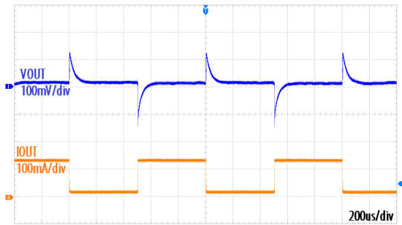
Output Load Transient without any Capacitor, V IN = 24V, V OUT = 12V
