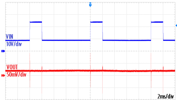
Line Transient Without Output Capacitor, V OUT = 3.3V, I OUT = 10mA
