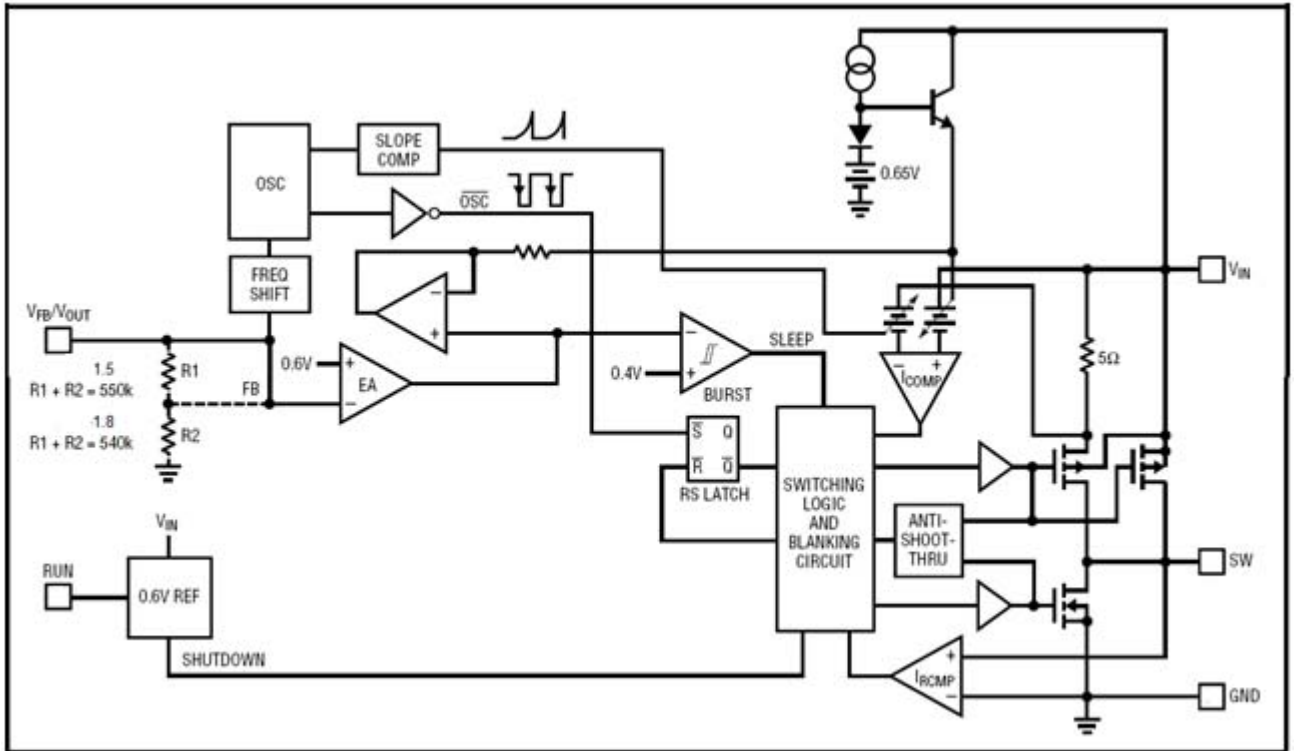
Figure2:Functional Block Diagram of FTD6811
