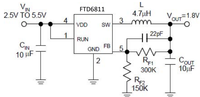
Figure 3. Type Application Circuit of FTD6811
