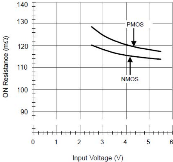
RDS(ON) vs Input Voltage
