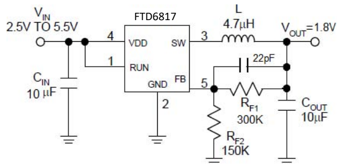
Figure 3. Type Application Circuit of FTD6817
