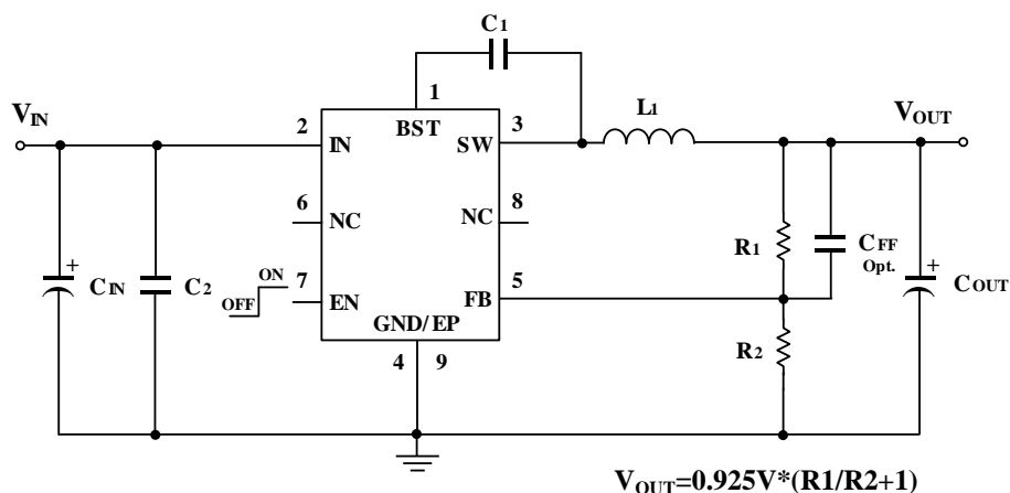
Figure 1 - Schematic Diagram
