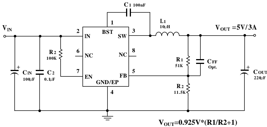
Figure 2 - 5V Output Application Circuit
