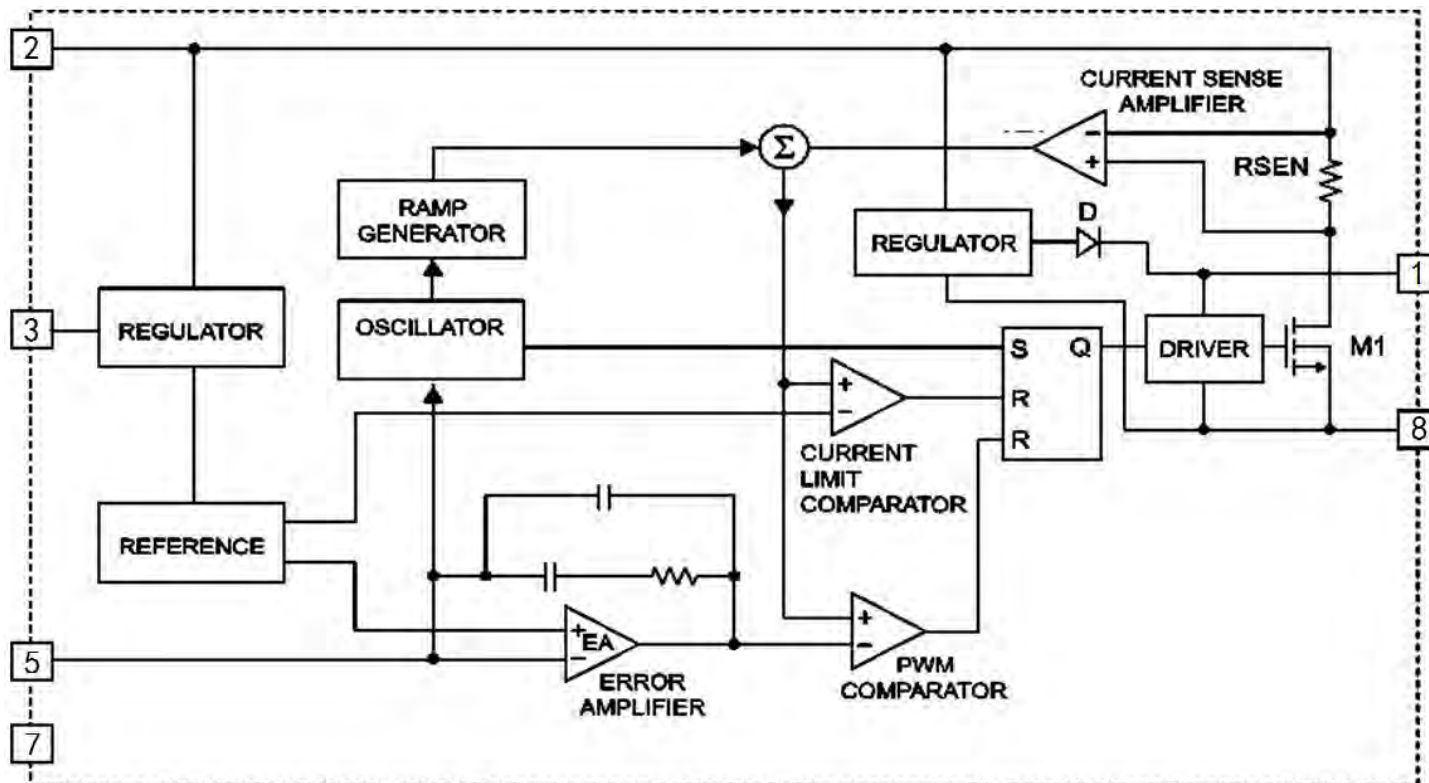
Figure 1 Function Block Diagram of FTD1468
