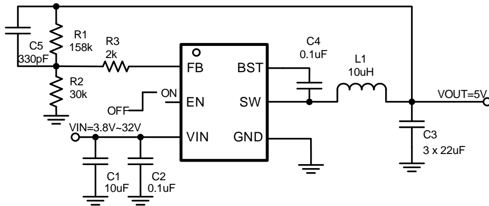
Figure 13. 24V Input, 5V/3A Output
