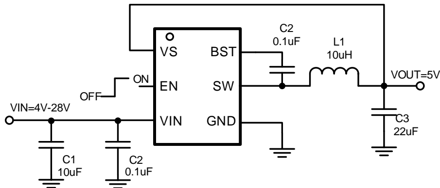
Figure 23. FC2325 Typical Application
