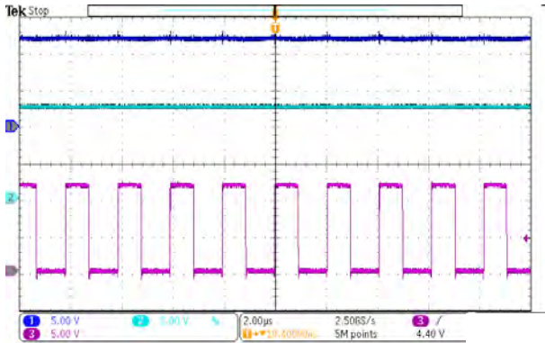
Figure 11. FC2332 Switching Node Waveform
