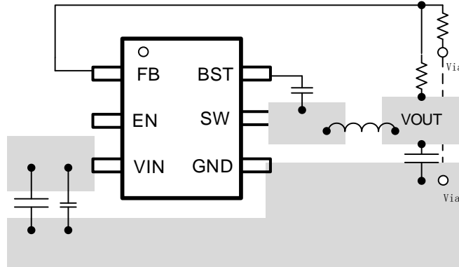
Figure 22. PCB Layout Example
