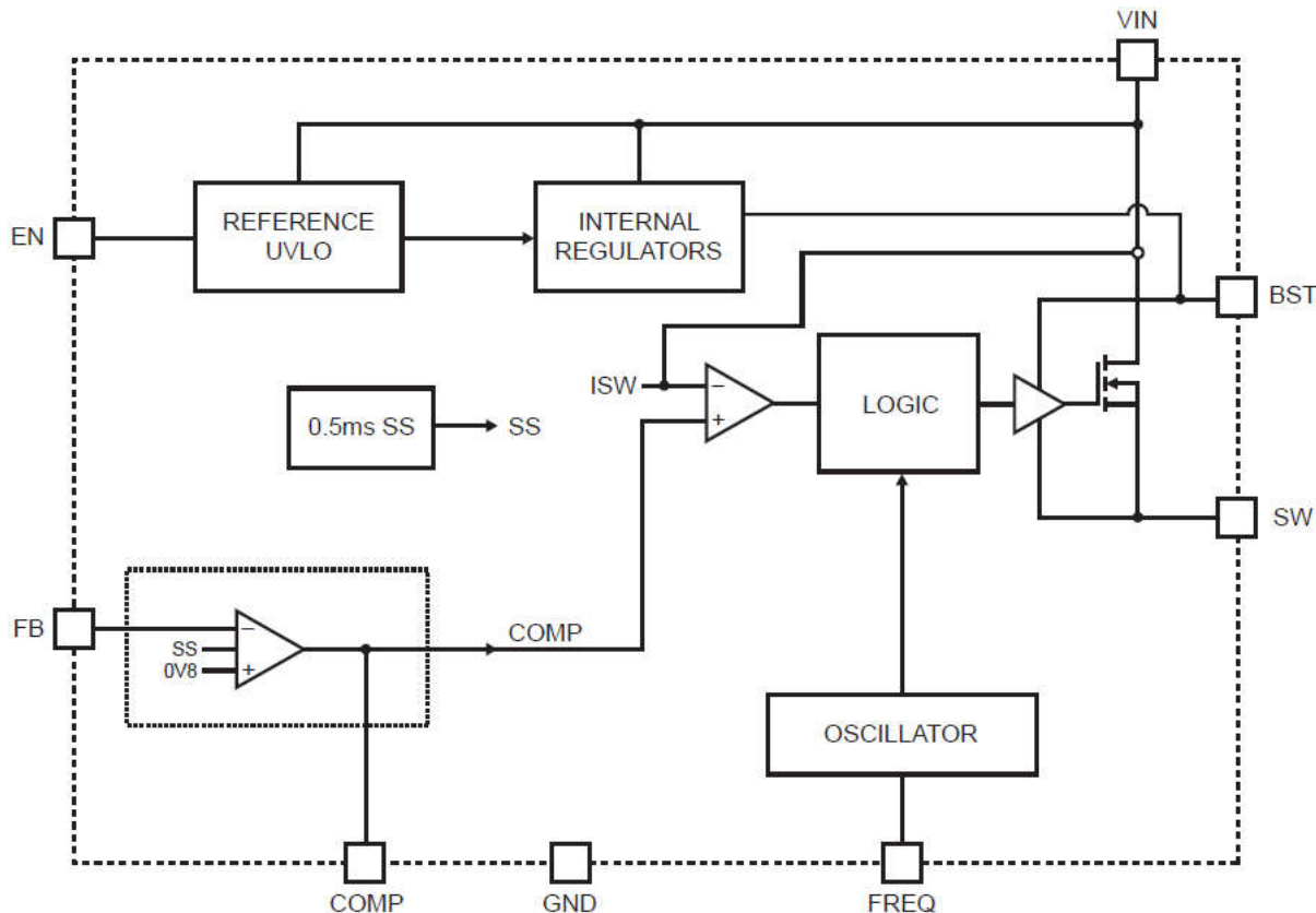
Figure1 Function Block Diagram of FTD1660
