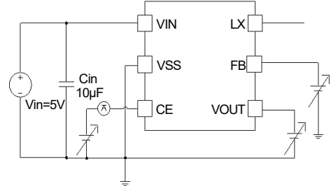
Circuit No.4
