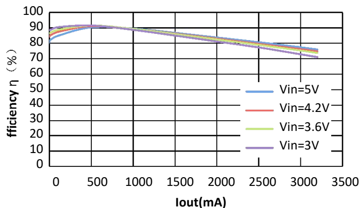
Iout vs Efficiency(Vout=1.2V)
