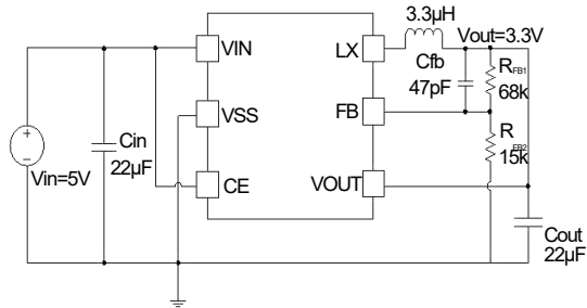
Circuit No.3
