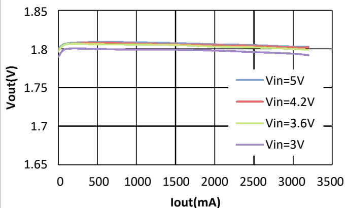
Iout vs Vout(Vout=1.8V)
