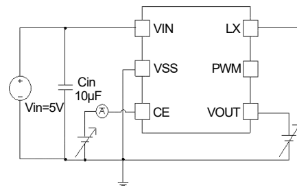
Circuit No.4
