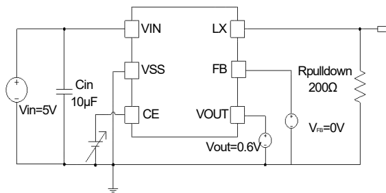
Circuit No.5
