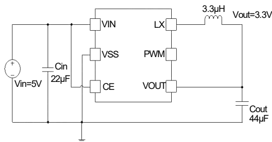
Circuit No.3
