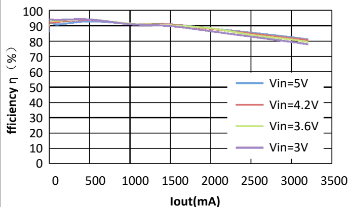
Iout vs Efficiency(Vout=1.8V)
