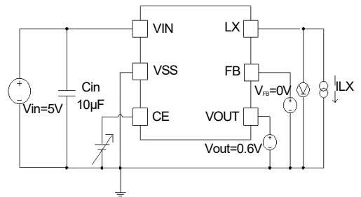
Circuit No.4
