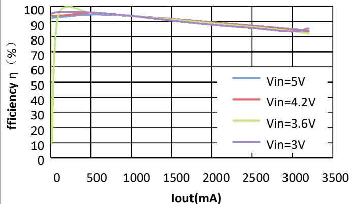
Iout vs Efficiency(Vout=2.5V)
