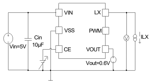
Circuit No.4
