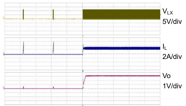
Short circuit recovery (20ms/div)
