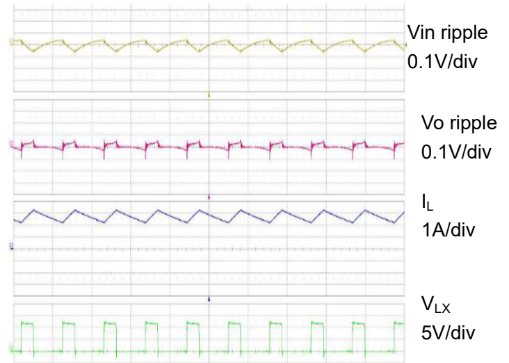
Full load operation (2 \mu\text{s}/\text{div} )
