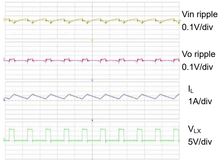
Light load operation (2 \mu\text{s}/\text{div} )
