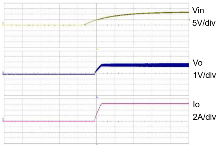
Start up to full load (10ms/div)
