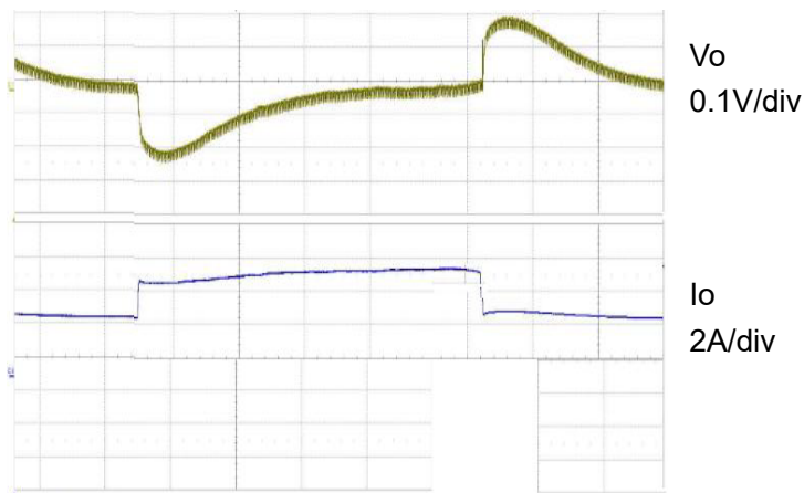
50% to 100% load transient (10 \mu\text{s}/\text{div} )
