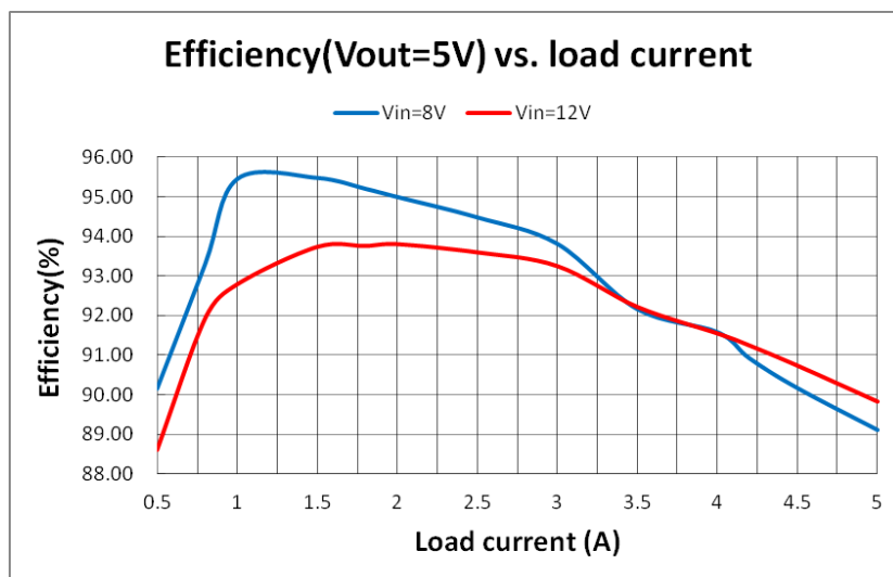
Fig.2 Efficiency1 (Vout=5V)
