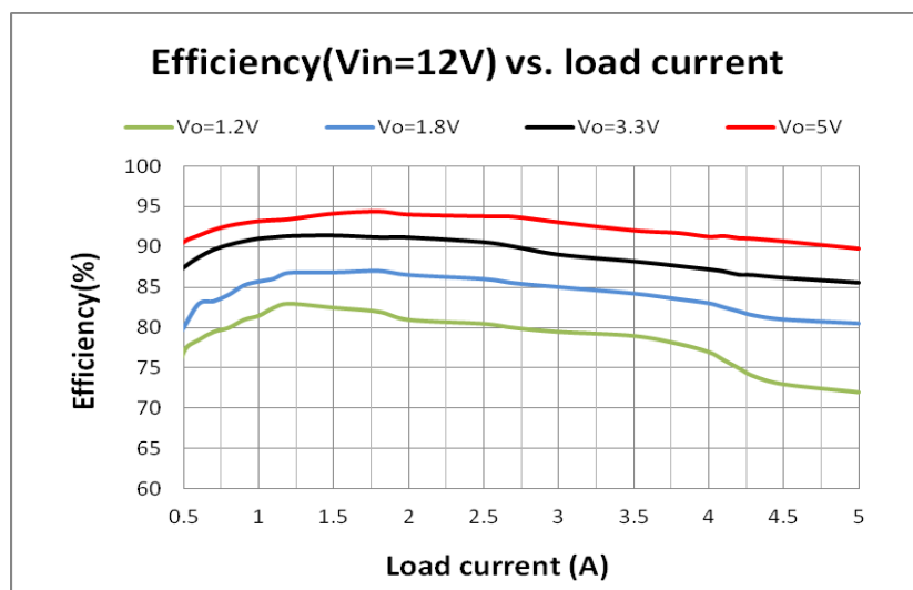
Fig.3 Efficiency2 (Vin=12V)
