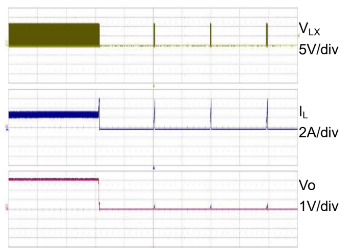
Short circuit protection (20ms/div)
