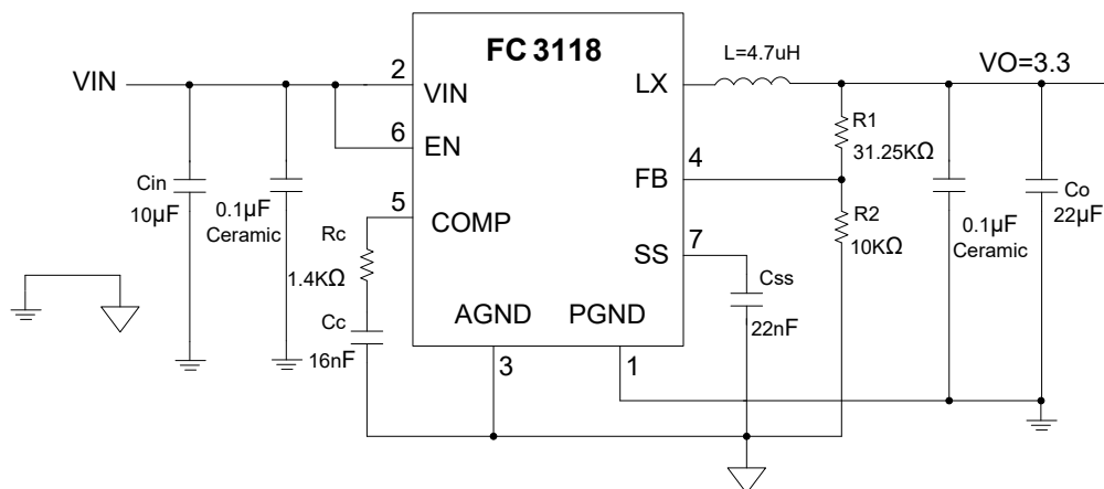
Fig.1 3.3V 3A Synchronous Buck Regulator, F_s = 500 \text{ KHz}
