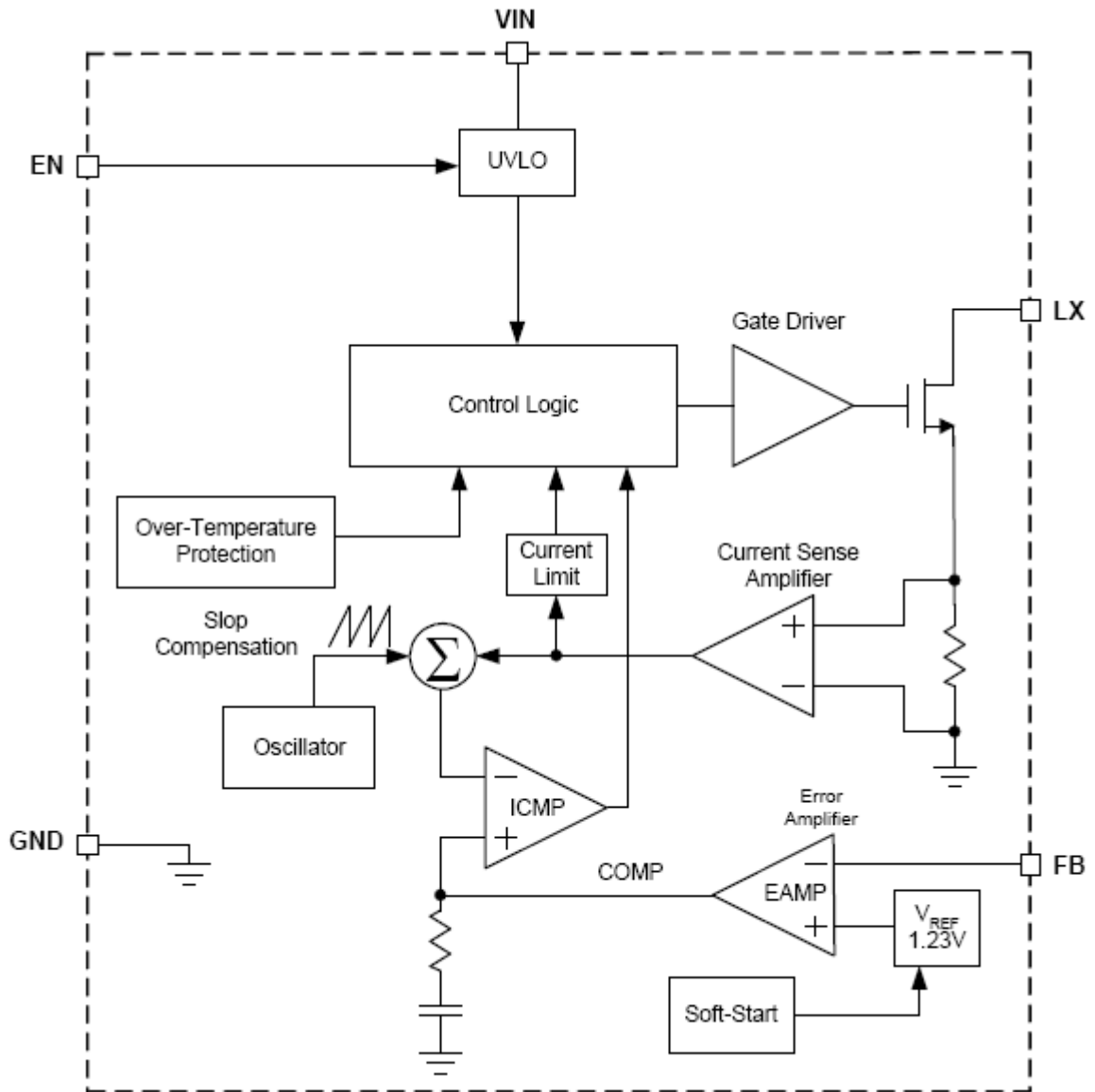
Figure 3 Function Block Diagram of FTD8210
