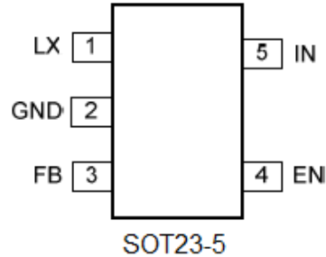
Figure 2 Pin Configuration of FTD8210(Top View)
