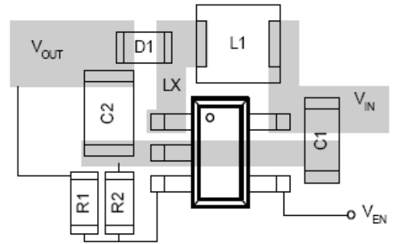
Optimized FTD8210 Layout
