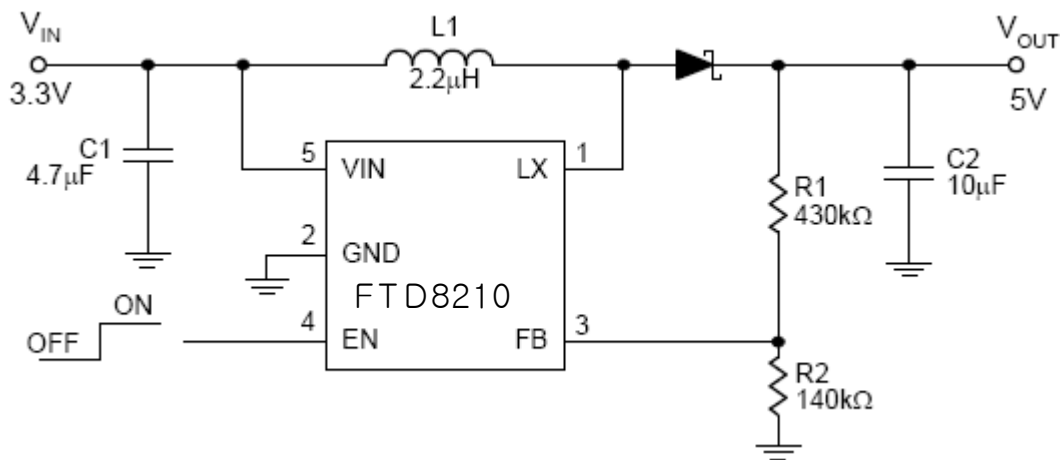
Figure 2. Standard 3.3V to 5V Supply
