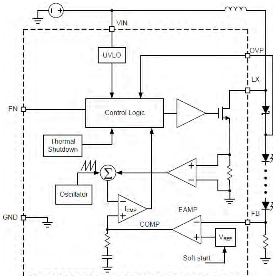
Functional Block Diagram of FTD8203
