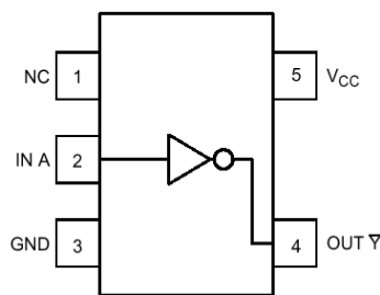
Figure 1. Pinout (Top View)
