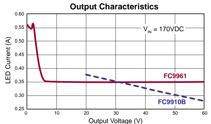
Fig.1. Typical output characteristic of an FC9961 LED driver.
