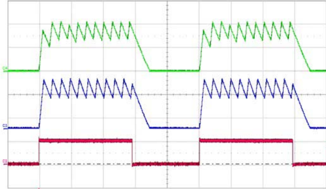
Fig.4. Typical PWM dimming response of an FC9961 LED driver.
