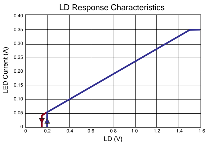
Fig.3. Typical linear dimming response of an FC9961 LED driver
