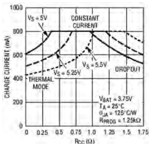
Figure 4: Charging current relationship with the RCC curve
