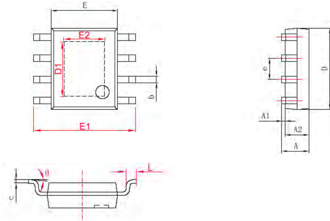
SOP-8E Package Outline Dimensions
