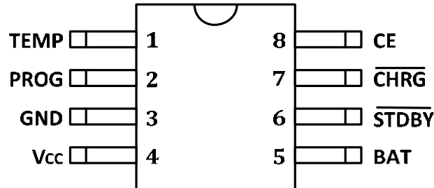
Figure 2 Pin Configuration of FC9056(Top View)
