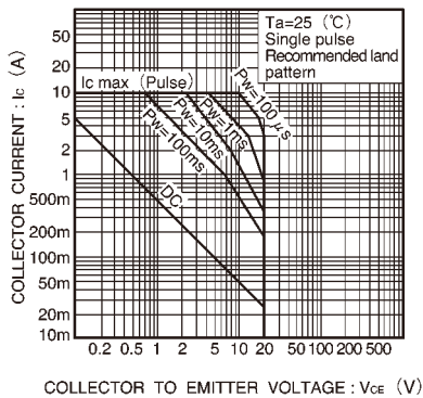
Fig.13 Safe operating area
