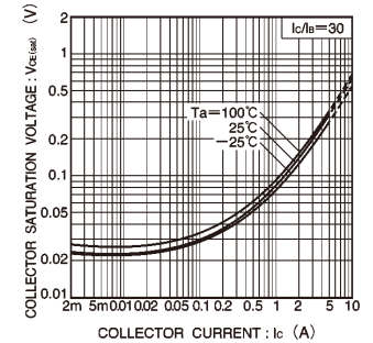
Fig.8 Collector-emitter saturation voltage vs. collector current ( III )
