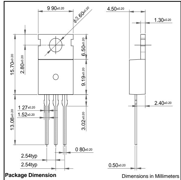
Package Dimension
