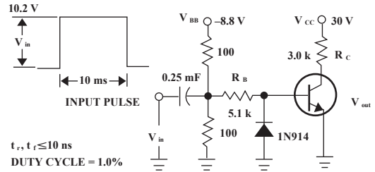
Values Shown are for I_C @ 10 \text{ mA} Figure 6. Switching Time Test Circuit
