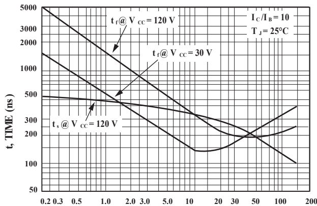
Figure 9. Turn-Off Time
