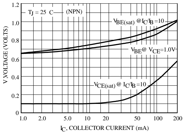
Figure 17. "ON" Voltages
