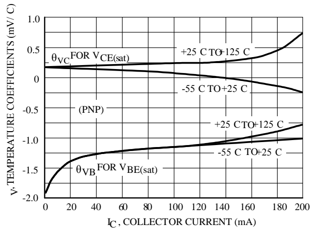
Figure 34. Temperature Coefficients
