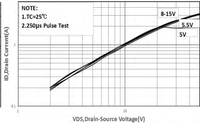
Fig2 Typical Output Characteristics, Tc=150°C
