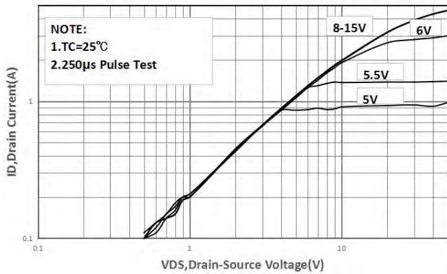
Fig1 Typical Output Characteristics, Tc=25°C
