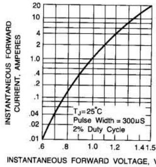
Fig. 1 - TYPICAL FORWARD CHARACTERISTICS
