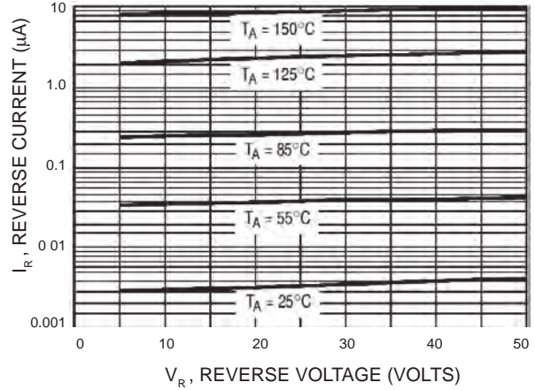
Figure 3. Leakage Current
