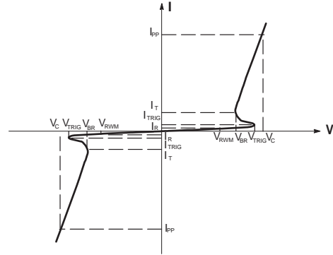
Bi-Directional TVS
