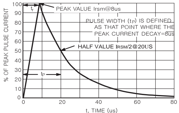
Figure 2. 8 x 20 \mu s Pulse Waveform
