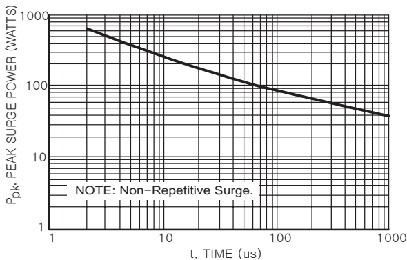
Figure 1. Pulse Width
