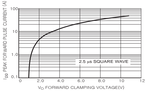
Figure 7. Clamping Voltage versus Peak Pulse Current (Forward Direction)
