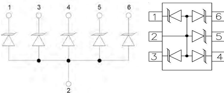
Circuit and Pin Schematic
