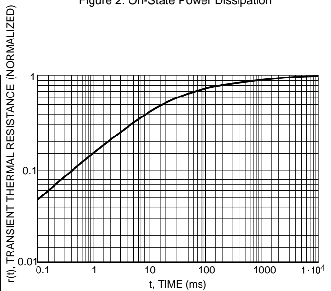
Figure 4. Thermal Response
