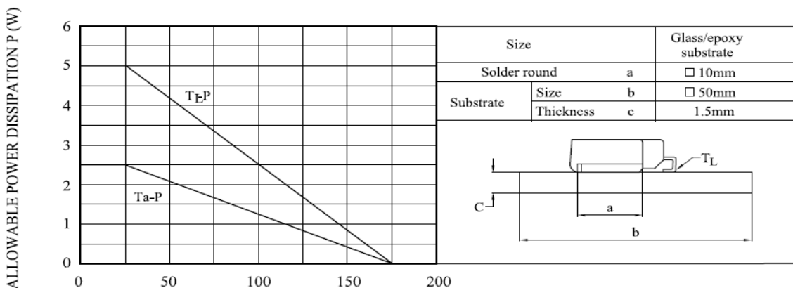
Fig. 5- LEAD TEMPERATURE T L , AMBIENT TEMPERATURE T a (°C)
