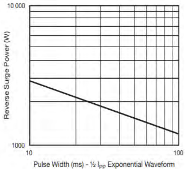
Fig. 4 - Reverse Power Capability
