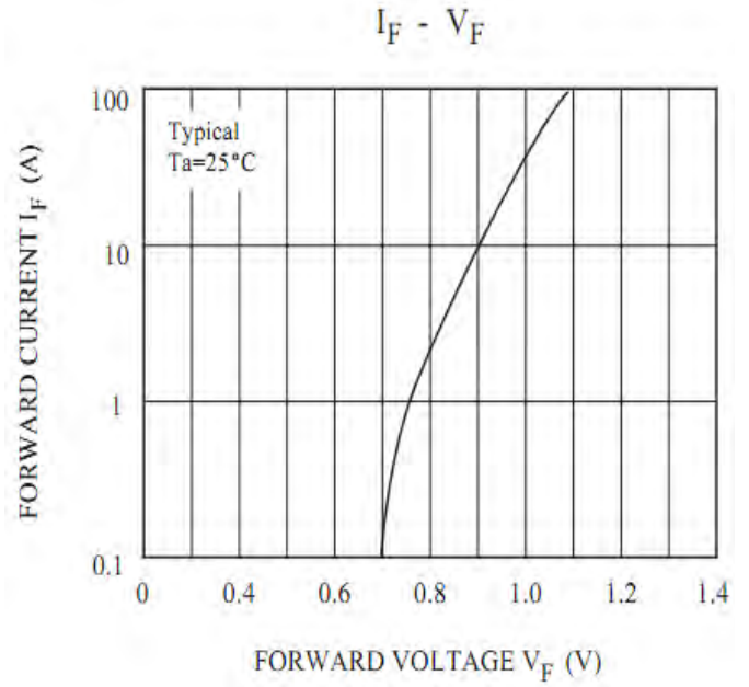
Fig. 7-Typical Forward Current
