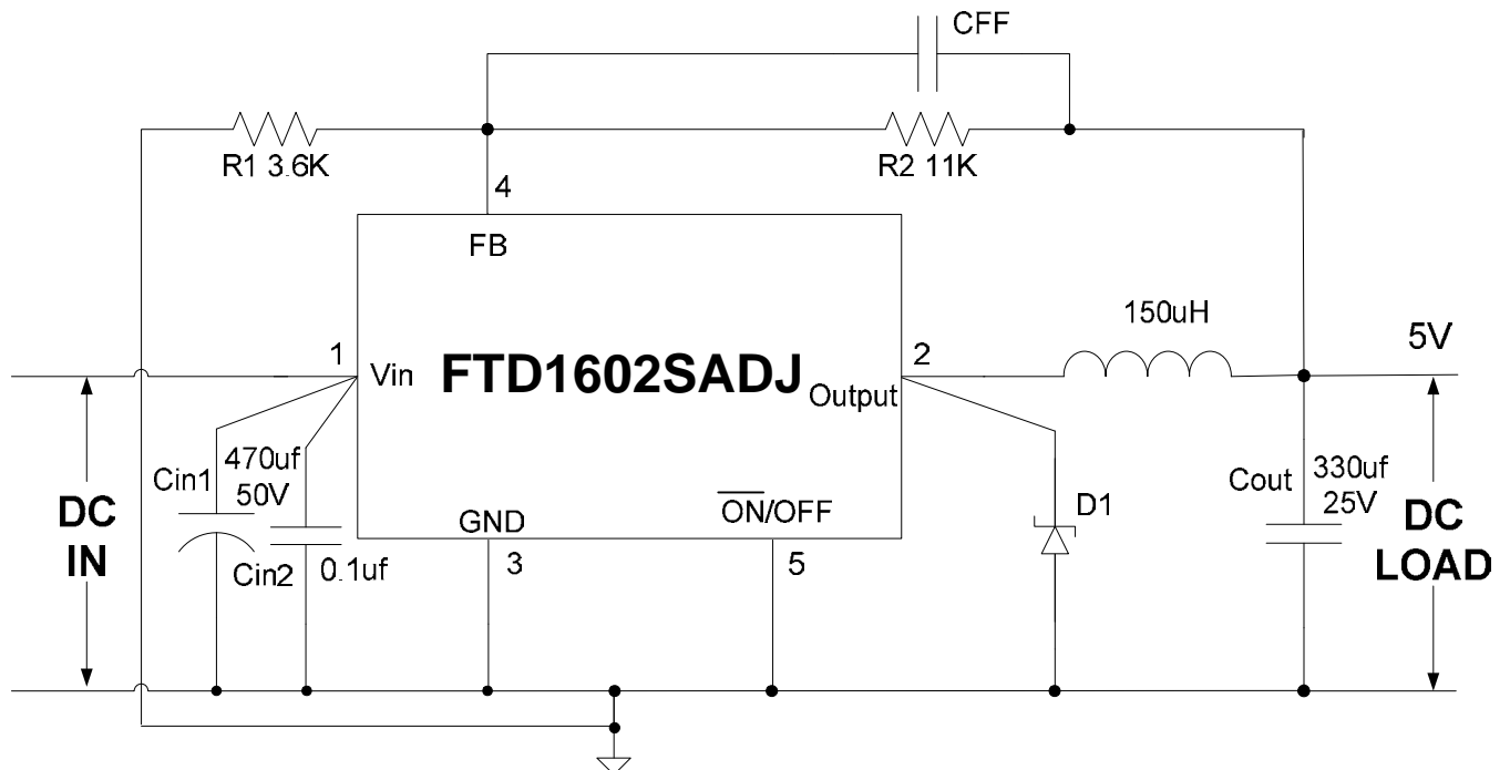
Figure 12. Typical Application of FTD1602 For ADJ
