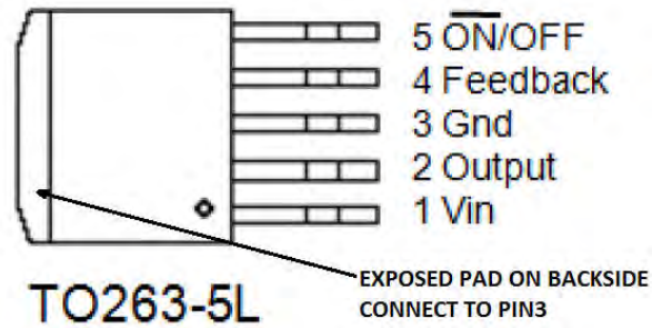
Figure 2. Pin Configuration of FTD1602 (Top View)
