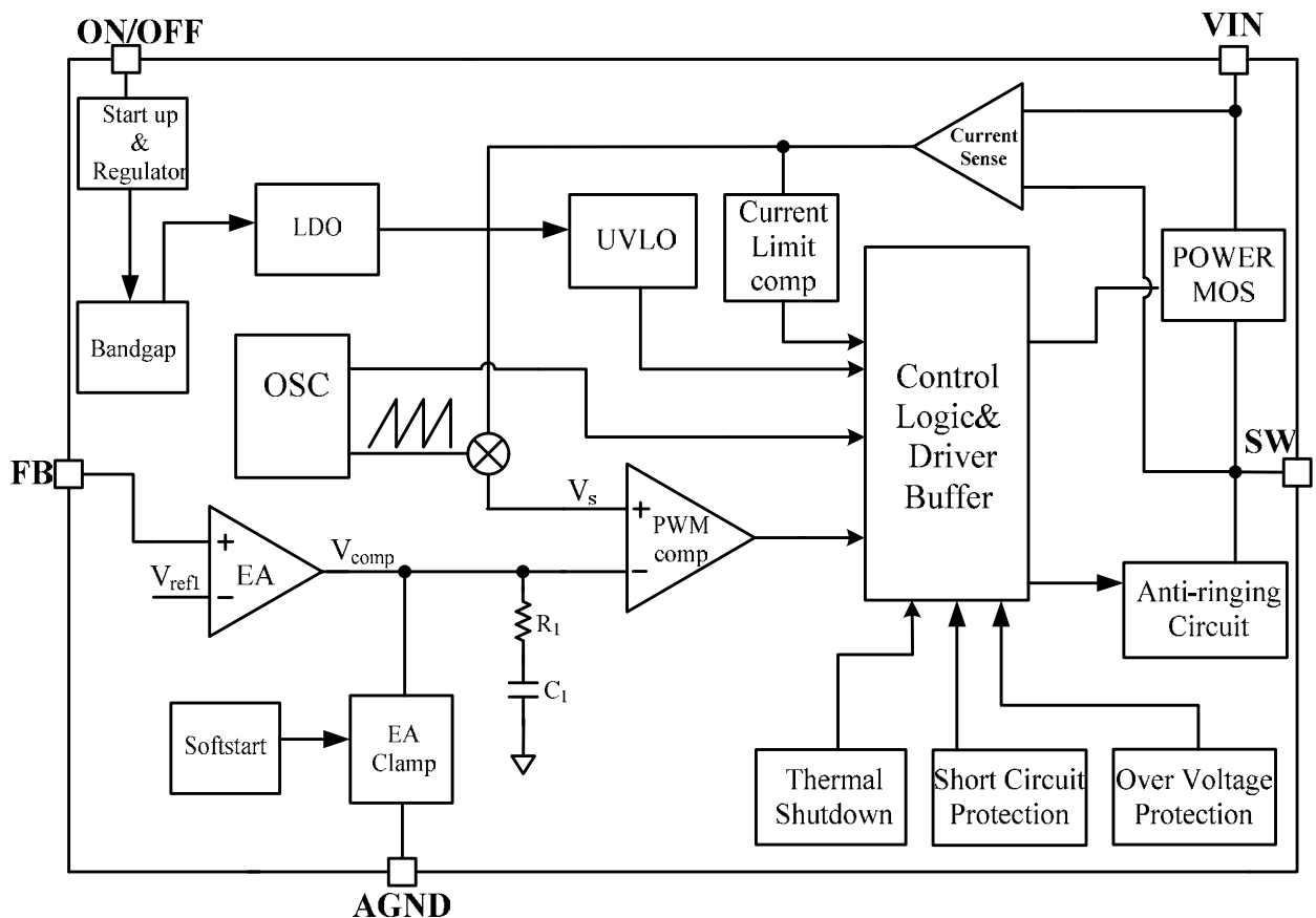
Figure3. Function Block Diagram of FTD1602
