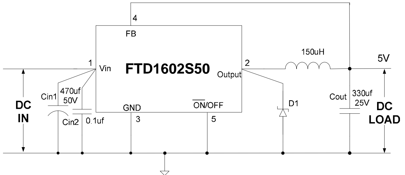
Figure 11. Typical Application of FTD1602 For 5V
