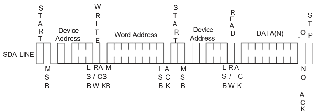
Figure 7: Random Read
