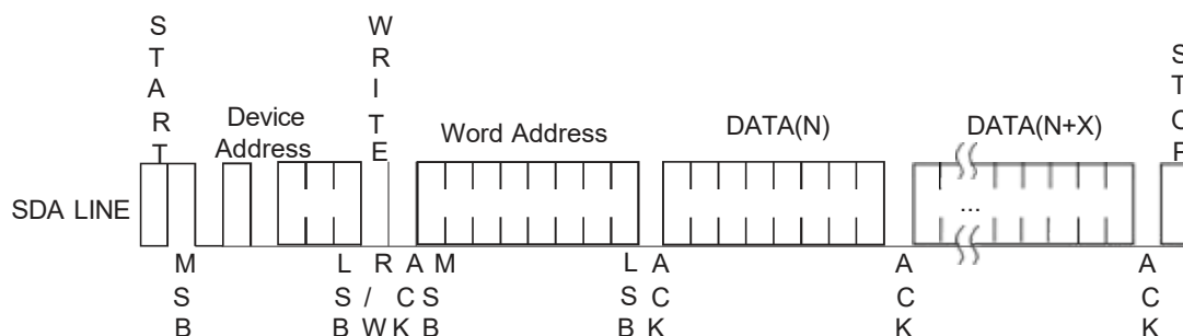
Figure 4: Page Write
