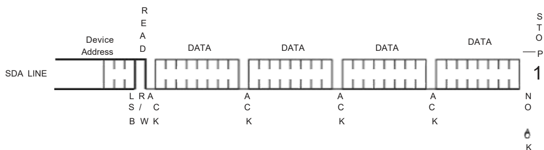
Figure 6: Sequential Read
