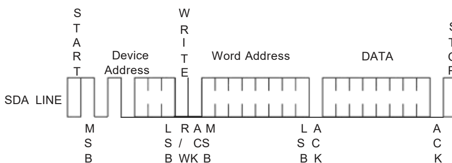
Figure 3: Byte Write
