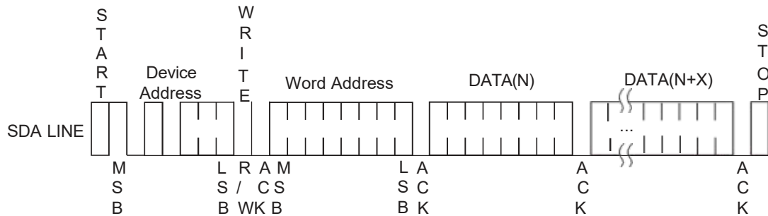
Figure 4: Page Write
