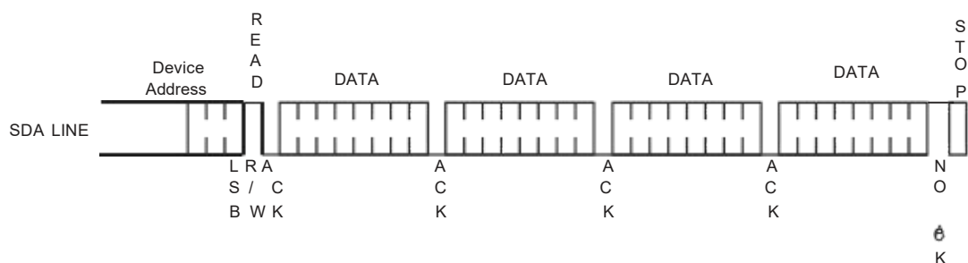
Figure 6: Sequential Read
