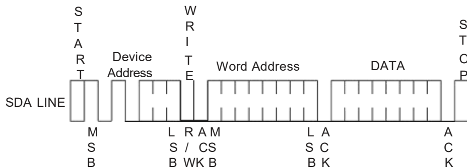
Figure 3: Byte Write
