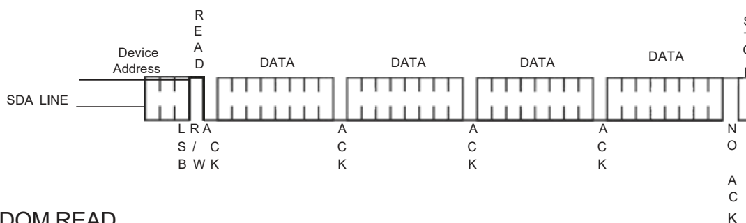
Figure 6: Sequential Read
