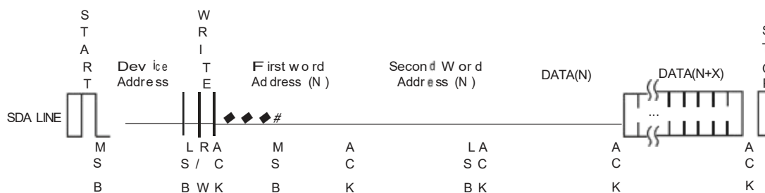
Figure 4: Page Write
