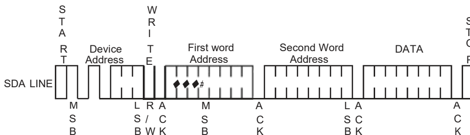
Figure 3: Byte Write
