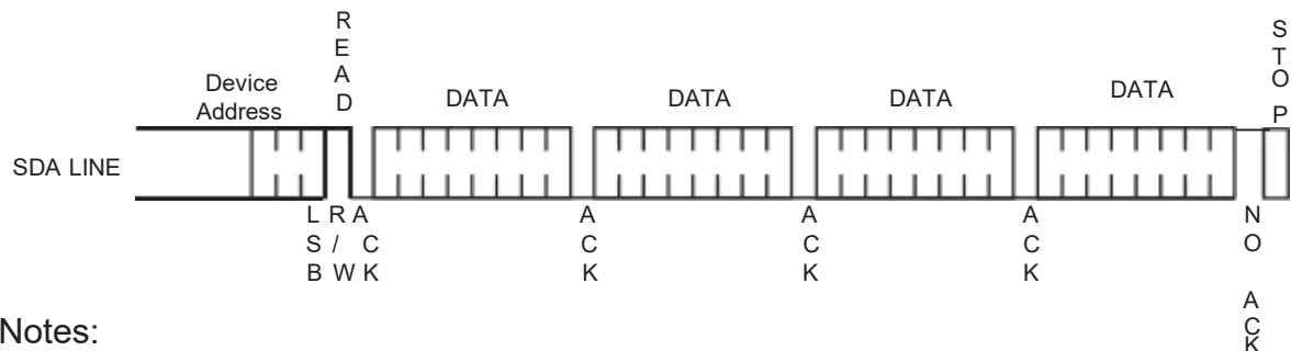
Figure 6: Sequential Read
