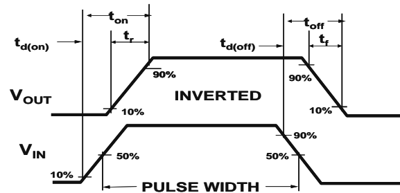
Figure 2: S switching Waveforms
