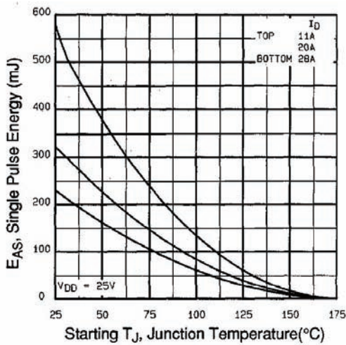
Fig. 11 - Maximum Avalanche Energy vs. Drain Current
