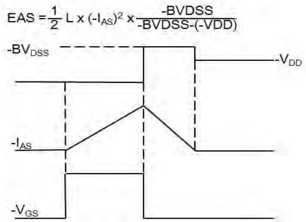
Fig.8 EAS Waveform
