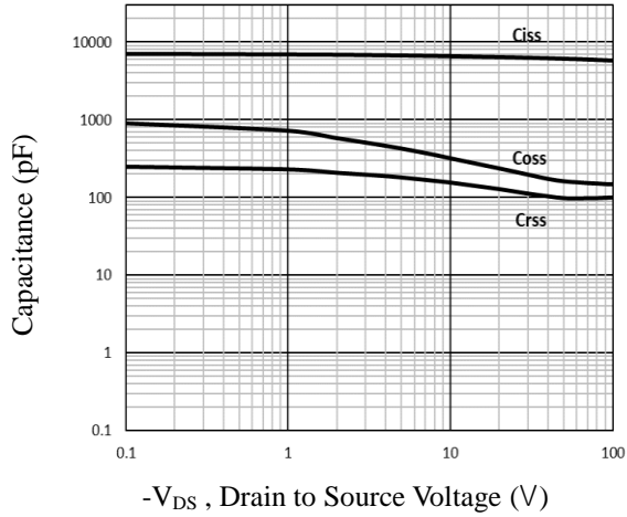
Fig.7 Capacitance Characteristics
