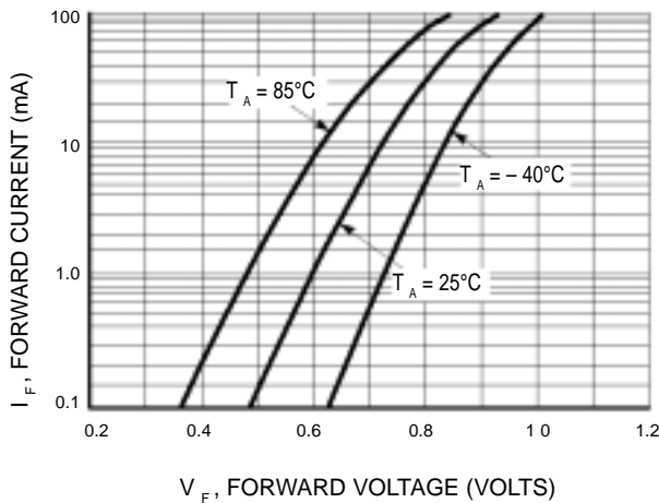
Figure 2. Forward Voltage
