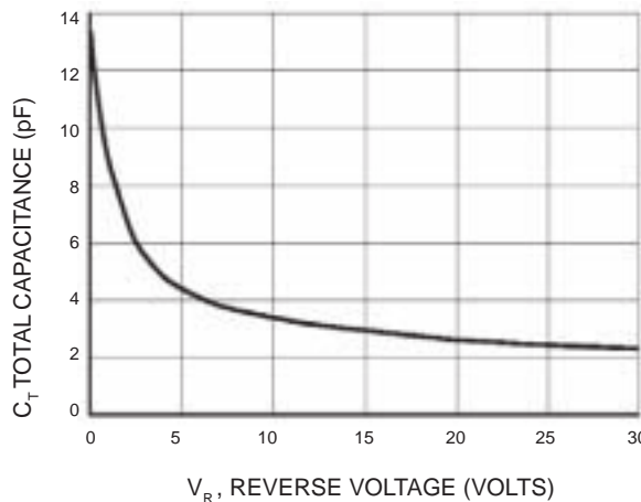
Figure 4. Total Capacitance
