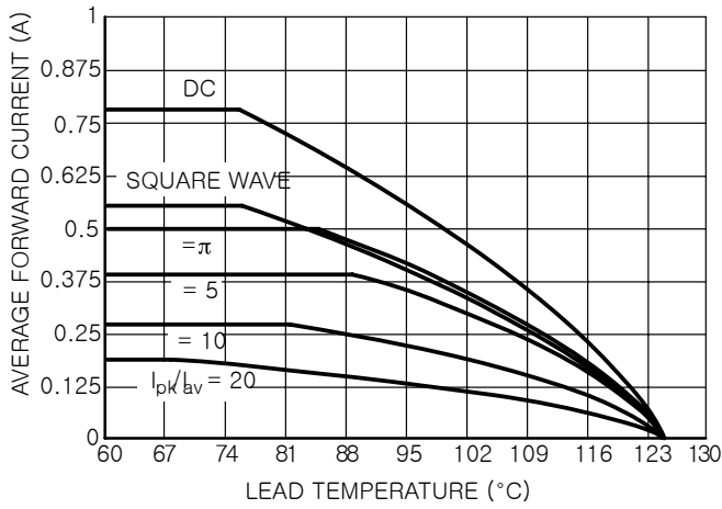
Figure 4. Current Derating (Lead)
