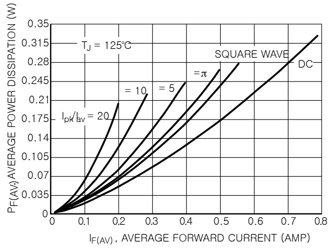
Figure 5. Power Dissipation
