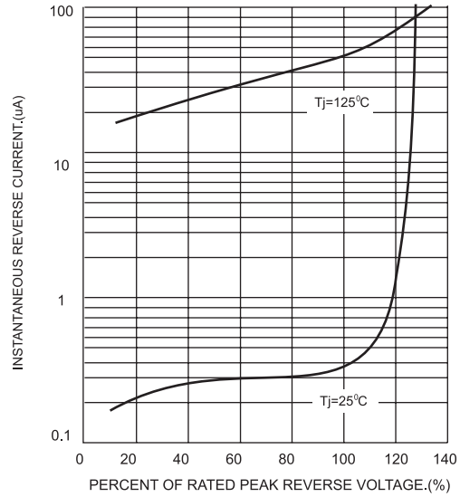
FIG.4-TYPICAL REVERSE CHARACTERISTICS
