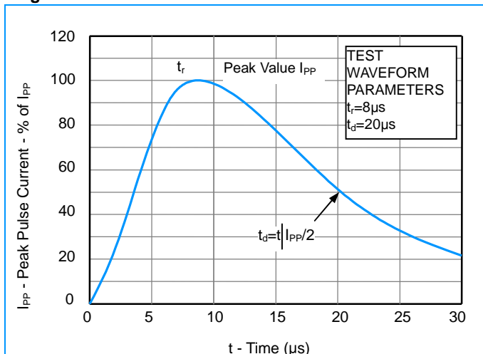
Fig1. 8/20s Pulse Waveform
