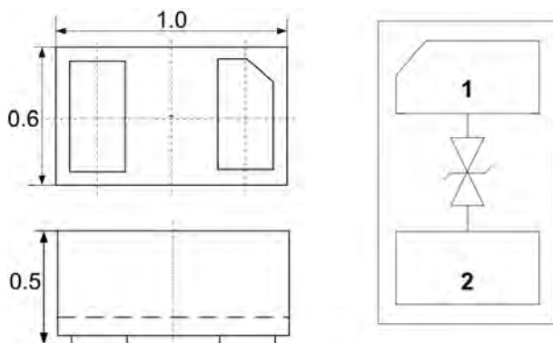
Package Dimensions
