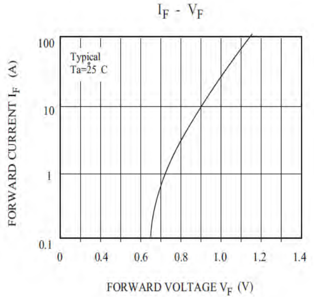
Fig. 7-Typical Forward Voltage
